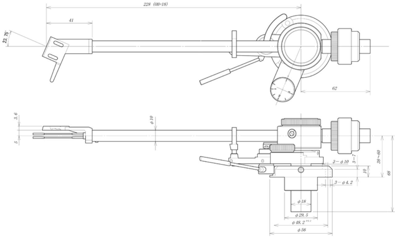
SA-250ST DRAWING
